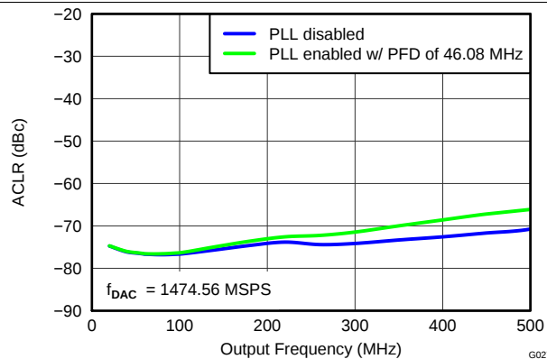
Figure 27. Single-Carrier WCDMA ACLR (Adjacent) vs Output Frequency Over Clocking Options
