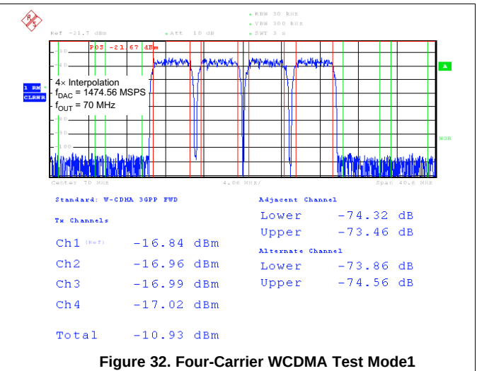
Figure 32. Four-Carrier WCDMA Test Mode1
