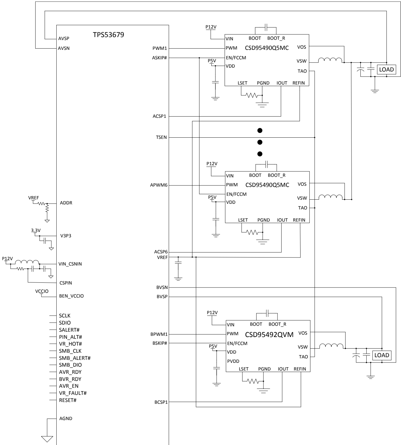
Figure 1. Application Schematic
