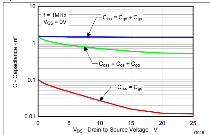
Figure 16. Control MOSFET Capacitance
