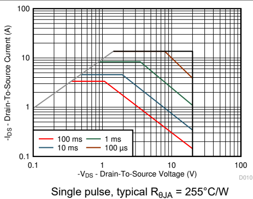
図 4-10. Maximum Safe Operating Area
