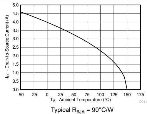
図 4-11. Maximum Drain Current vs Temperature
