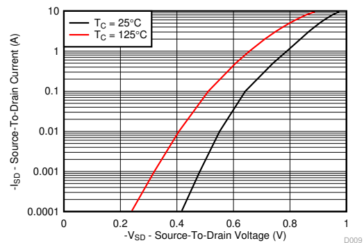
図 4-9. Typical Diode Forward Voltage
