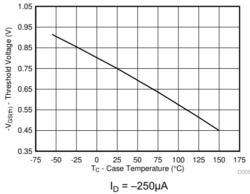
図 4-6. Threshold Voltage vs Temperature
