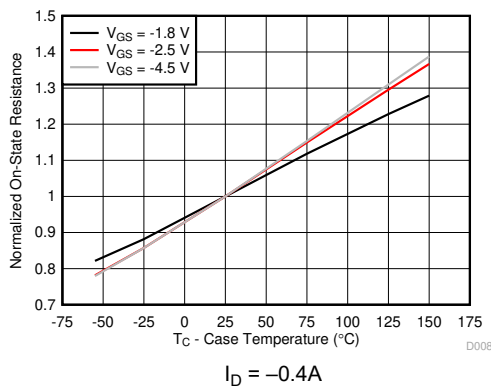
図 4-8. Normalized On-State Resistance vs Temperature
