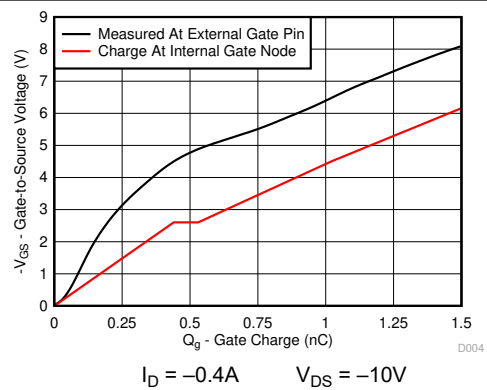
Figure 4-4. Gate Charge
