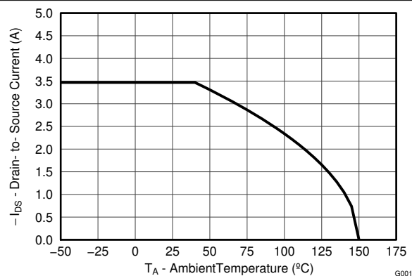
FIG 5-11. Maximum Drain Current vs Temperature
