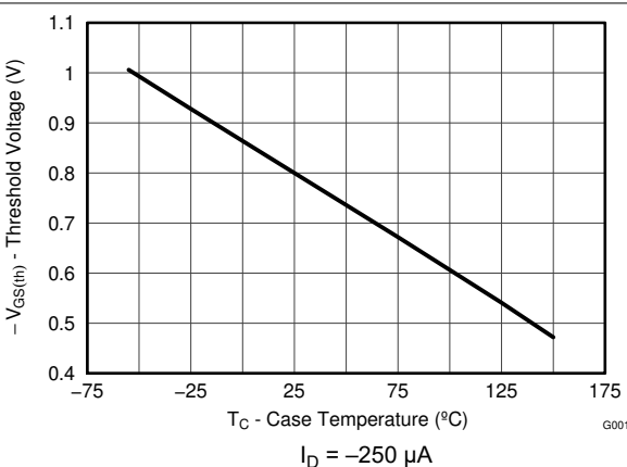
FIG 5-6. Threshold Voltage vs Temperature
