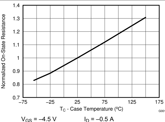
FIG 5-8. Normalized On-State Resistance vs Temperature
