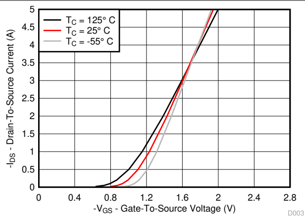
5-2. Transfer Characteristics
