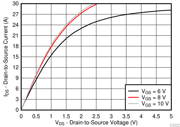
図 3-2. Saturation Characteristics
