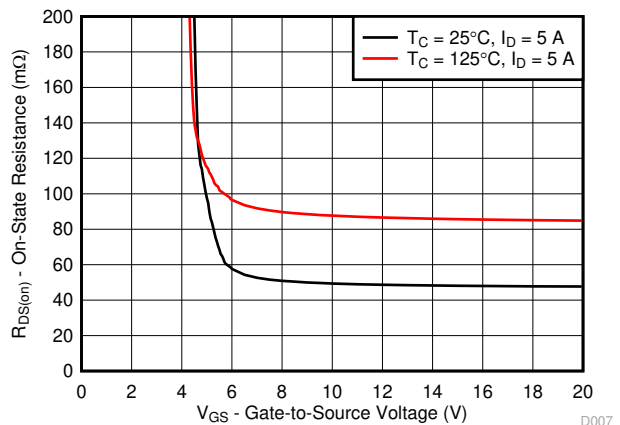
図 3-7. On-State Resistance vs Gate-to-Source Voltage
