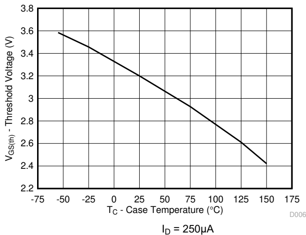
図 3-6. Threshold Voltage vs Temperature
