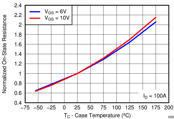
FIG 4-8. Normalized On-State Resistance vs Temperature
