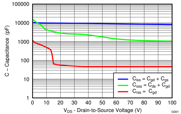
FIG 4-5. Capacitance
