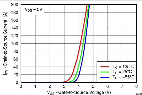
図 4-3. Transfer Characteristics
