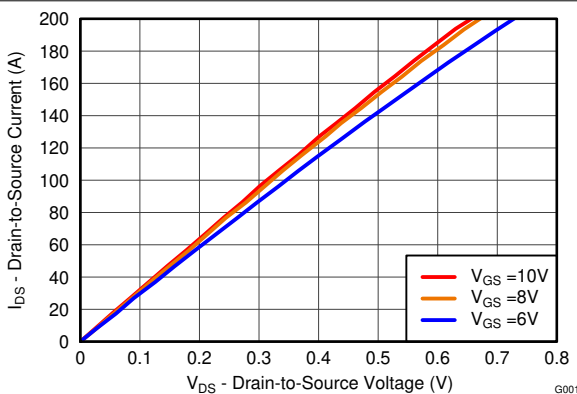
図 4-2. Saturation Characteristics
