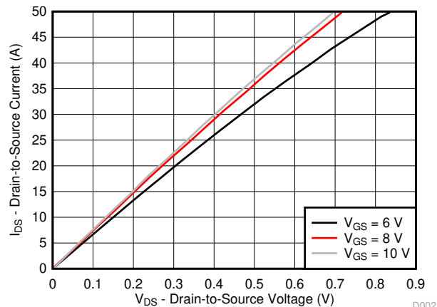
图 4-2. Saturation Characteristics
