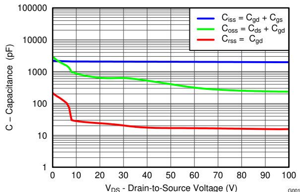
4-5. Capacitance
