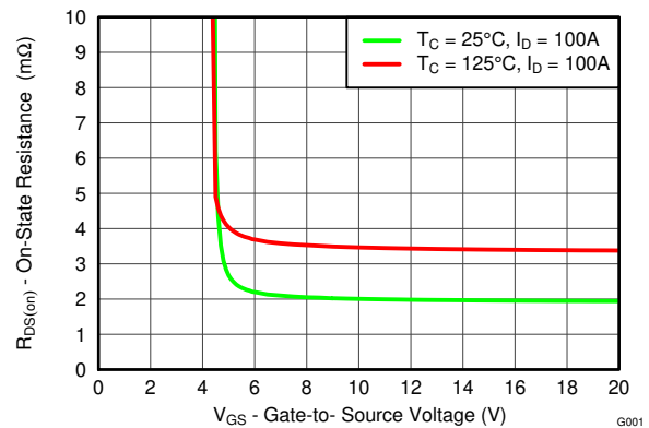
図 4-7. On-State Resistance vs Gate-To-Source Voltage
