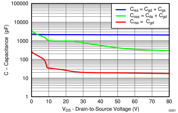
4-5. Capacitance
