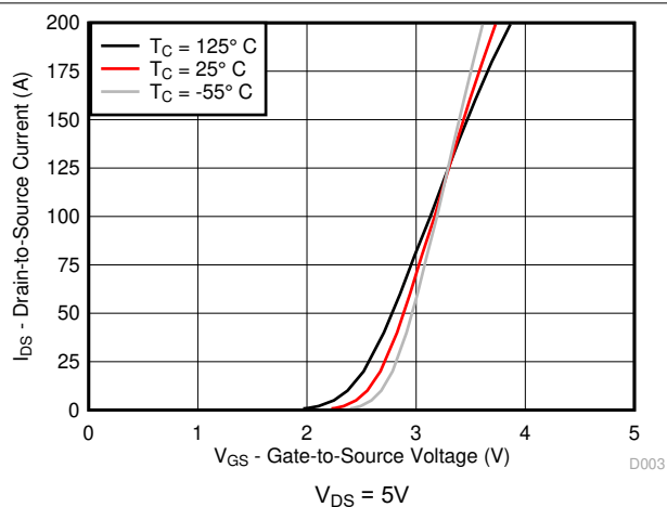
図 4-3. Transfer Characteristics
