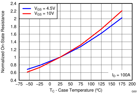
3-8. Normalized On-State Resistance vs Temperature
