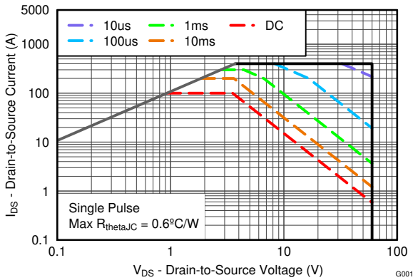
3-10. Maximum Safe Operating Area
