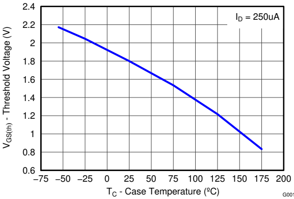
3-6. Threshold Voltage vs Temperature
