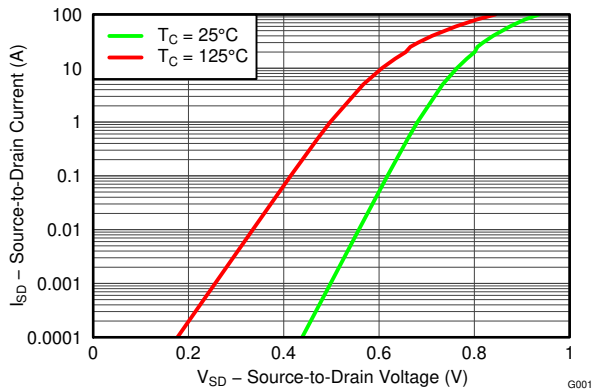
3-9. Typical Diode Forward Voltage
