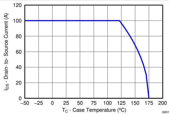
3-12. Maximum Drain Current vs Temperature
