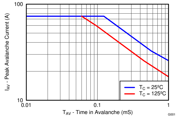
3-11. Single Pulse Unclamped Inductive Switching
