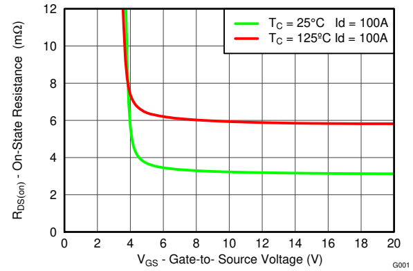
3-7. On-State Resistance vs Gate-to-Source Voltage
