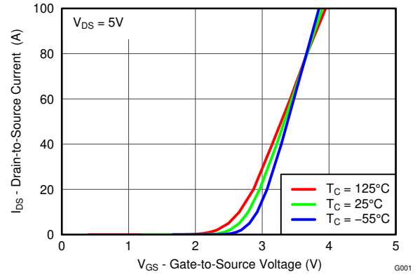
4-3. Transfer Characteristics
