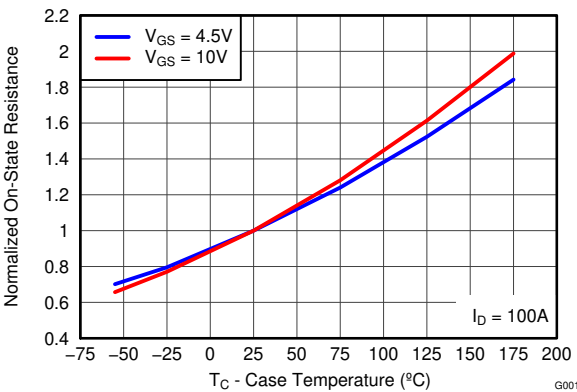
図 4-8. Normalized On-State Resistance vs. Temperature
