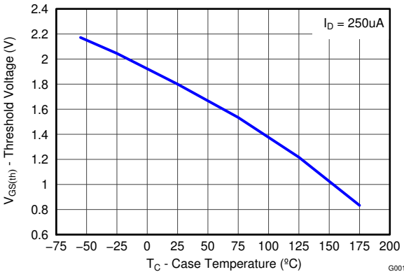
図 4-6. Threshold Voltage vs. Temperature
