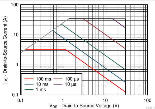
FIG 5-10. Maximum Safe Operating Area (SOA)
