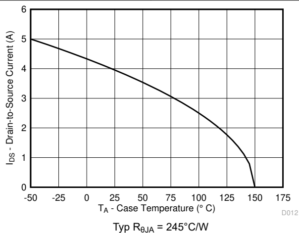
FIG 5-12. Maximum Drain Current vs Temperature
