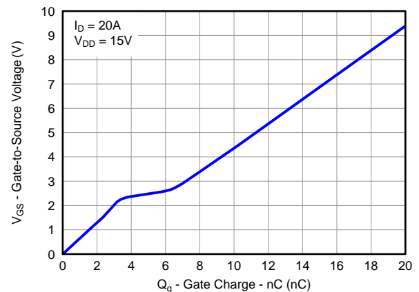
GATE CHARGE
