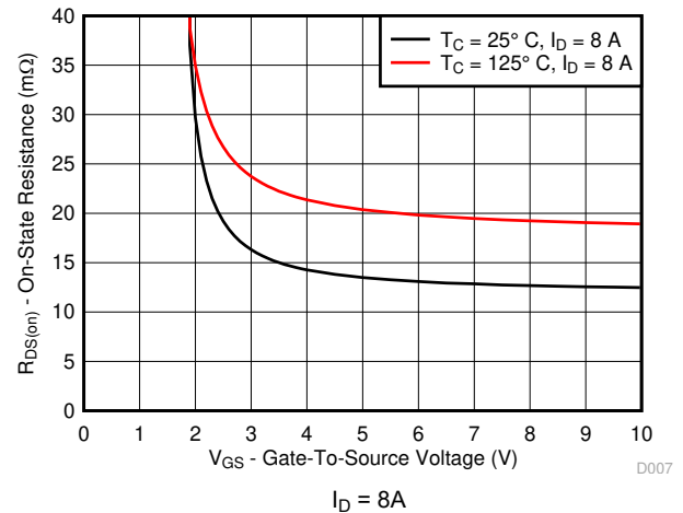
図 4-7. On-State Resistance vs Gate-to-Source Voltage
