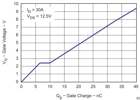
Figure 6-4. Gate Charge
