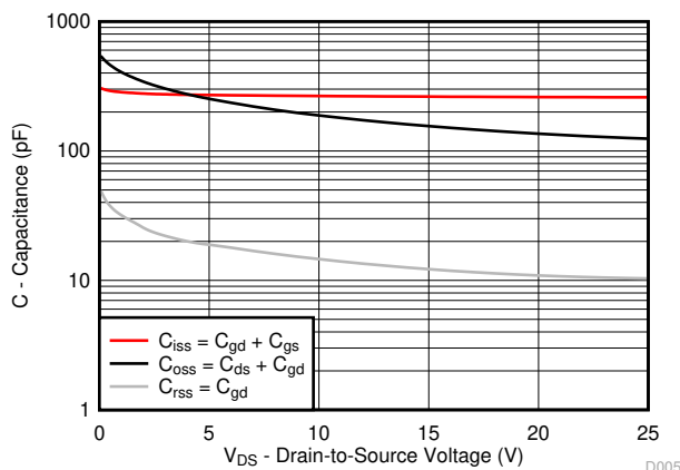
Figure 4-5. Capacitance
