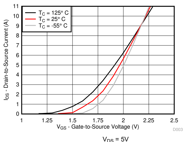
Figure 4-3. Transfer Characteristics
