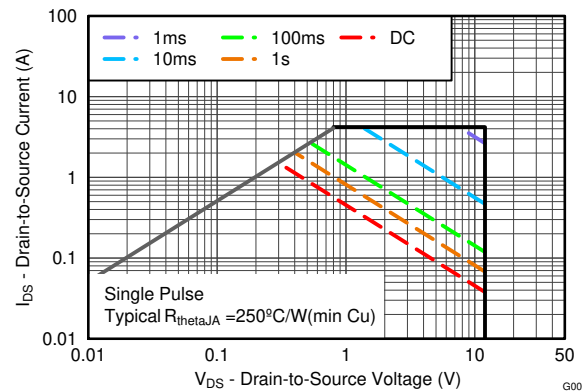
5-10. Maximum Safe Operating Area (SOA)
