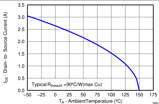
FIG 5-12. Maximum Drain Current vs Temperature
