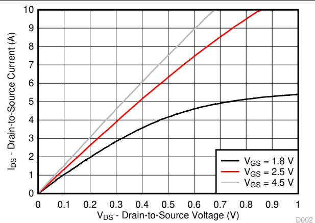
5-2. Saturation Characteristics
