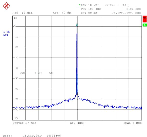
図 9-8. Output Spectrum With SSC Off
