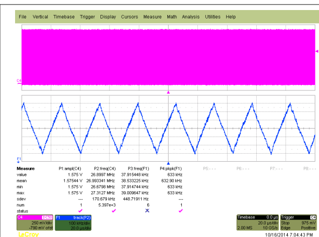
図 9-7. f_{out} = 27\text{MHz} , VCO frequency > 175MHz, SSC (1%, center)
