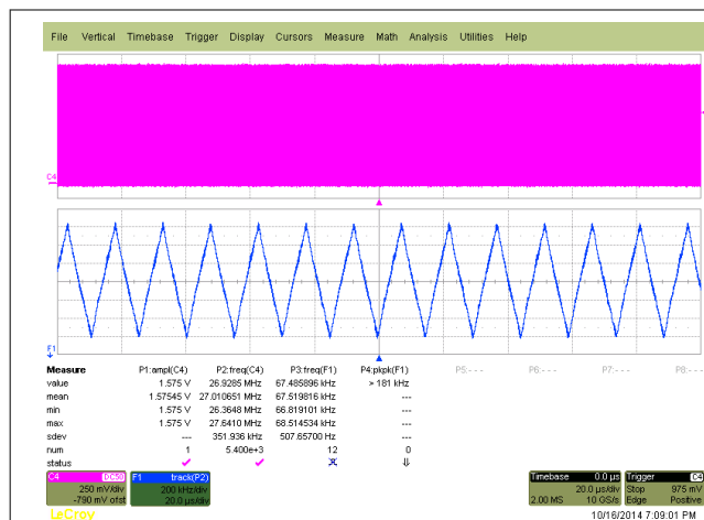
図 9-6. f_{out} = 27\text{MHz} , VCO frequency < 125MHz, SSC (2% center)
