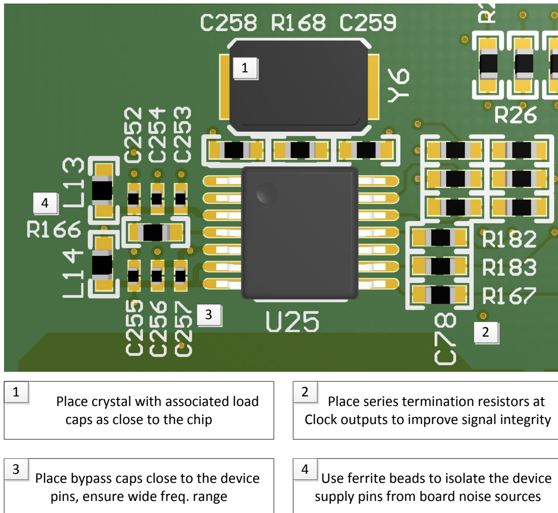
☒ 9-10. Annotated Layout
