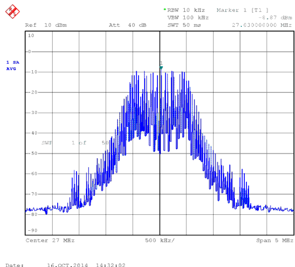
図 9-9. Output Spectrum With SSC On, 2% Center
