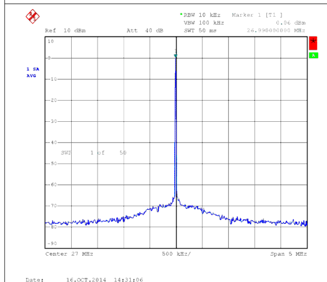
Figure 8-9. Output Spectrum With SSC Off
