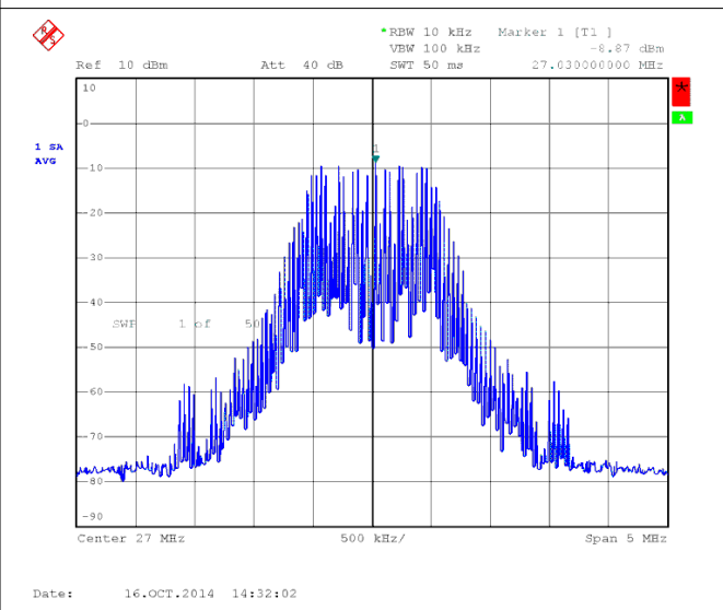
Figure 8-10. Output Spectrum With SSC On, 2% Center
