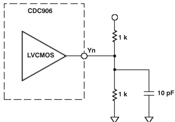
Figure 1. Test Load
