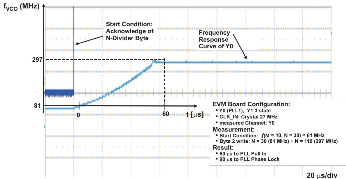
Figure 34. Snapshot of the PLL Lock-Time
