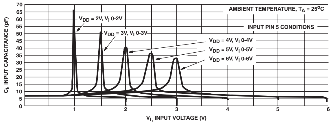
FIG 2. Input Capacitance as a Function of Input Voltage
