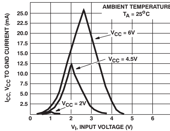
FIG 1. Typical Inverter Supply Current as a Function of Input Voltage
