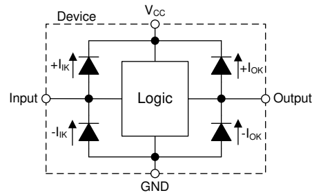
図 7. Electrical Placement of Clamping Diodes for Each Input and Output
