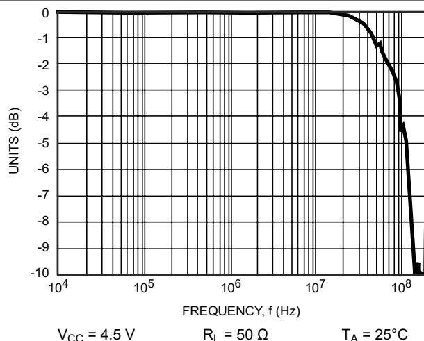
图 14-2. Typical Switch Frequency Response
