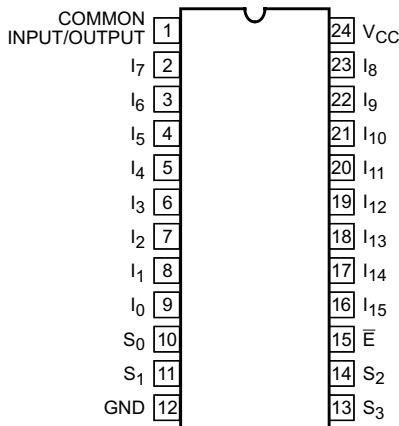
图 4-1. N, DW, or DB Packages 24-Pin PDIP, SOIC, or SSOP (Top View)
