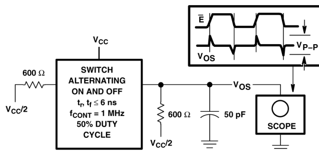
图 6-4. Control-to-Switch Feedthrough Noise Test Circuit
