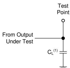
✎ 6-1. Load Circuit for Push-Pull Output
