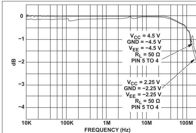
図 5-7. Channel ON Bandwidth (HC and HCT4053)
