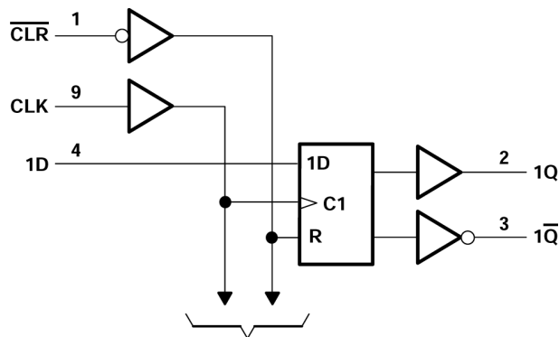
To Three Other Channels 論理図 (正論理)
