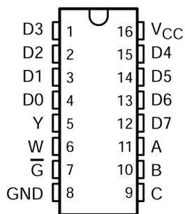
図 3-1. CD54ACT151 J Package; CD74ACT151 D or N Package; 16-Pin CDIP, SOIC, or PDIP (Top View)
