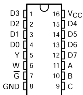
図 3-1. D or N Packages; 16-Pin SOIC or PDIP (Top View)
