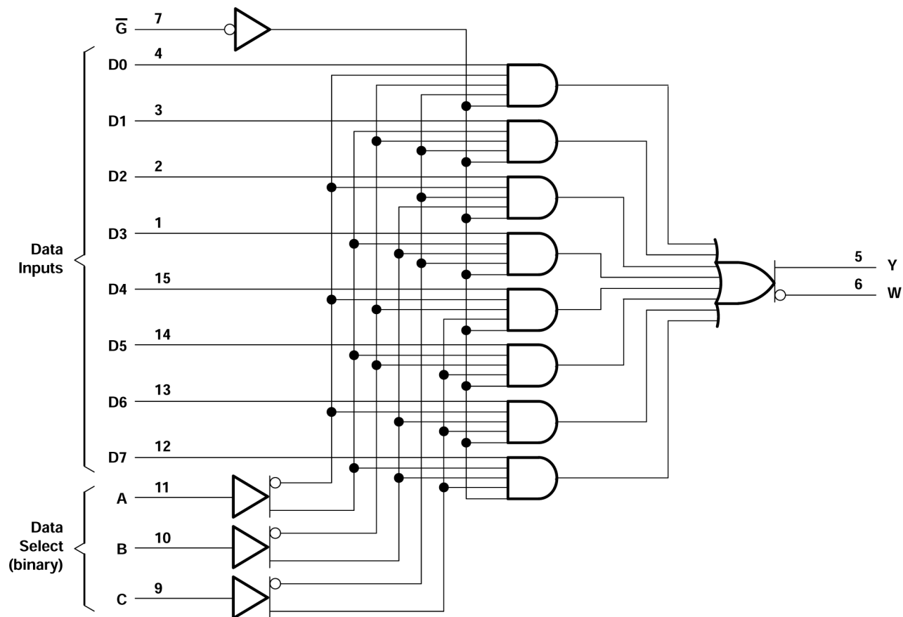
図 6-1. Logic Diagram (Positive Logic)
