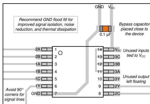
11-1. Example layout for the CD74HCT4075
