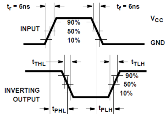
✎ 6-2. HC and HCT Transition Times and Propagation Delay Times, Combination Logic
