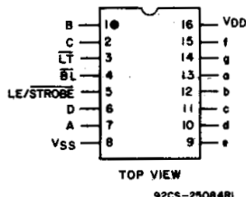
CD4511B TERMINAL ASSIGNMENT
