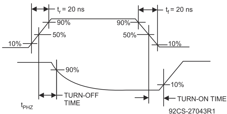
図 6-9. Propagation Delay Waveform Channel Being turned OFF ( R_L = 300\Omega , C_L = 50 \text{ pF} )
