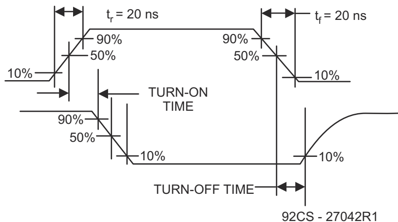
図 6-8. Propagation Delay Waveform Channel Being turned ON ( R_L = 10\text{k}\Omega , C_L = 50 \text{ pF} )
