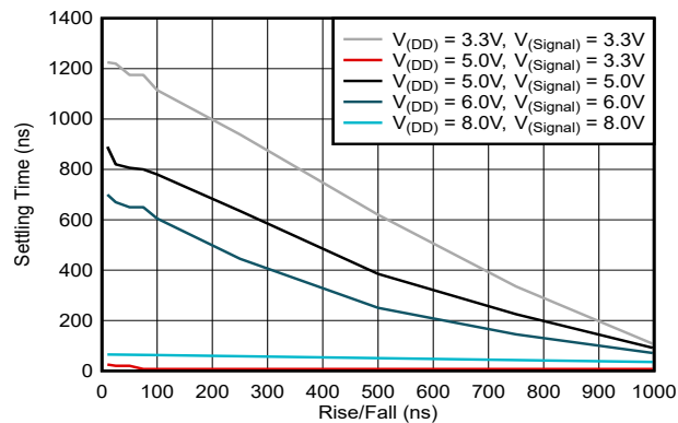
図 5-1. System Settling Time vs Signal Rise/Fall Time
