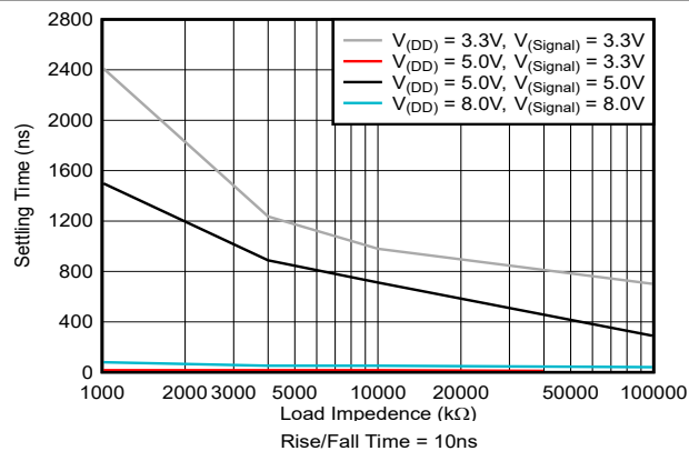
図 5-3. System Settling Time vs Signal Voltage
