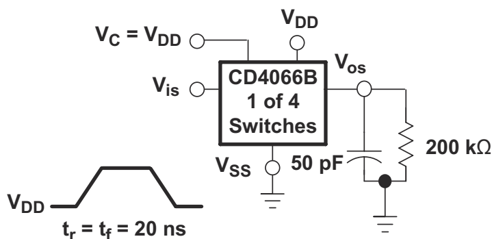
図 6-4. Off-Switch Input or Output Leakage
