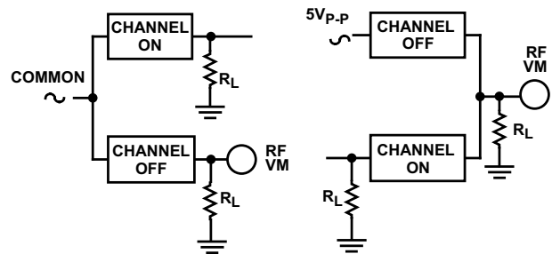
図 6-14. Crosstalk Between Any Two Channels (All Types)
