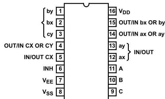
図 4-3. CD4053B E, M, NS, and PW Package, 16-Pin PDIP, CDIP, SOP, and TSSOP (Top View)
