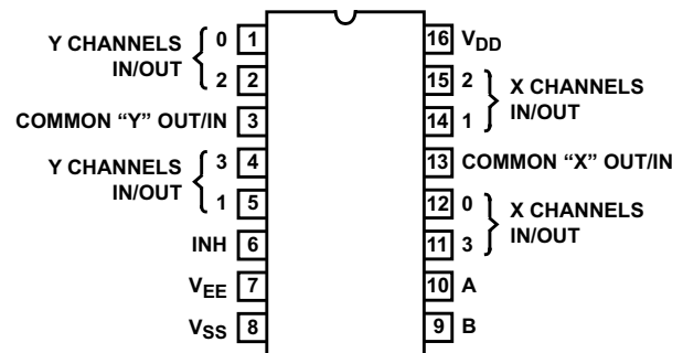
図 4-2. CD4052B E, M, NS, and PW Package, 16-Pin PDIP, CDIP, SOP, and TSSOP (Top View)
