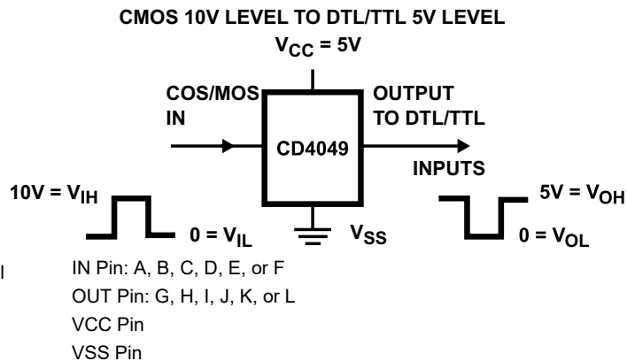
✎ 7-4. Logic Level Conversion Application
