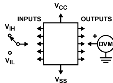
Fig 7-2. Input Voltage Test Circuit
