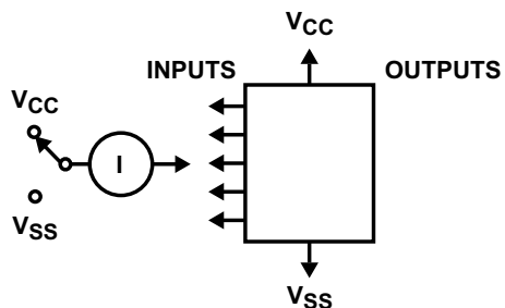
✎ 7-3. Input Current Test Circuit
