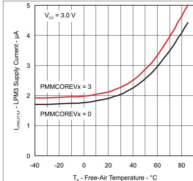
Figure 5-3. LPM3 Supply Current vs Temperature
