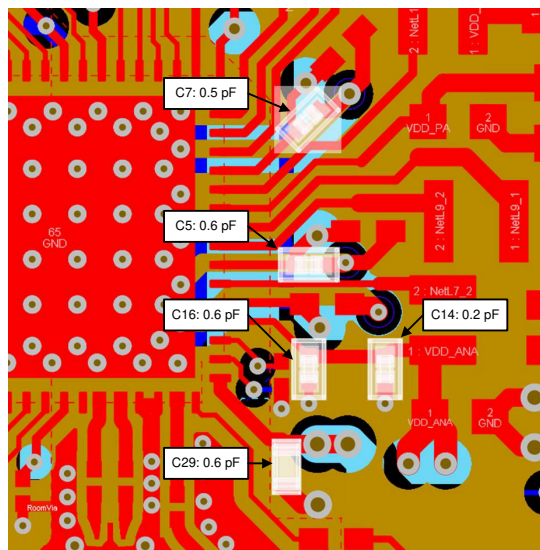
9-9. Ground Routing for Input Decoupling Capacitors
