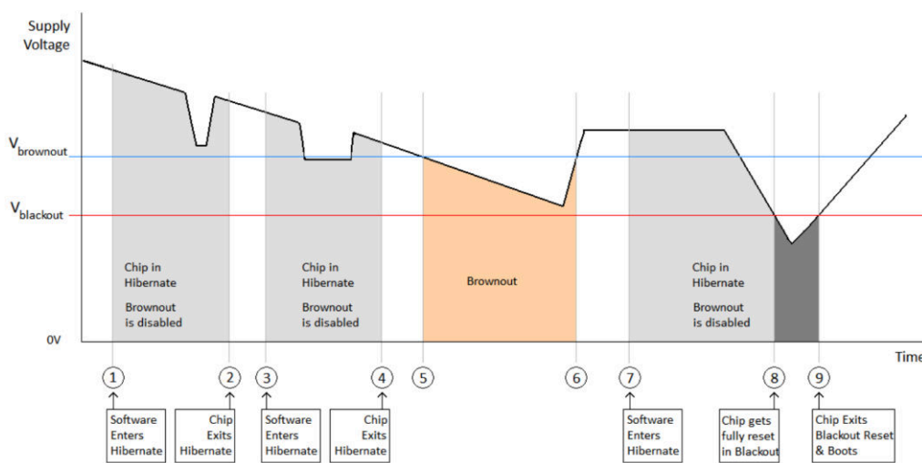
Figure 7-4. Brownout and Blackout Levels (1 of 2)
