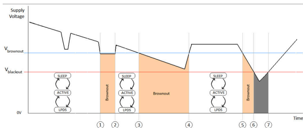
Figure 7-5. Brownout and Blackout Levels (2 of 2)
