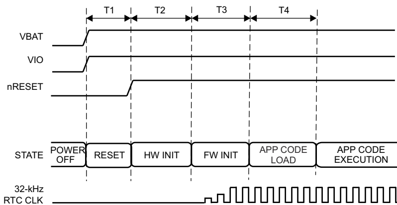
図 7-6. First-Time Power-Up and Reset Removal Timing Diagram (32kHz Crystal)
