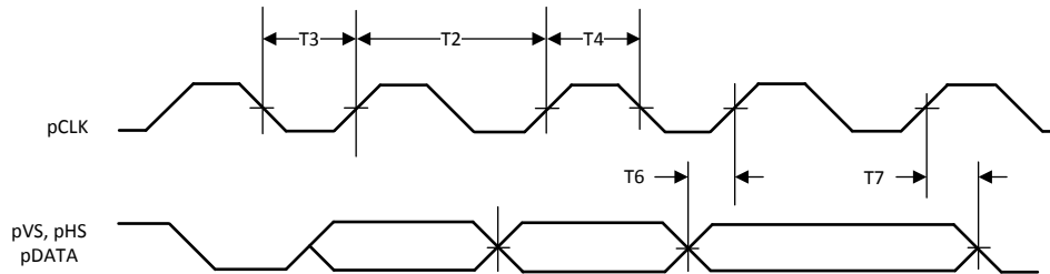
図 7-21. Camera Parallel Port Timing Diagram
