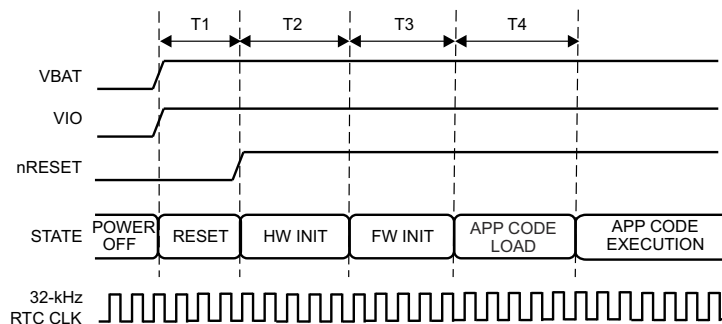
図 8-7. First-Time Power-Up and Reset Removal Timing Diagram (External 32-kHz)
