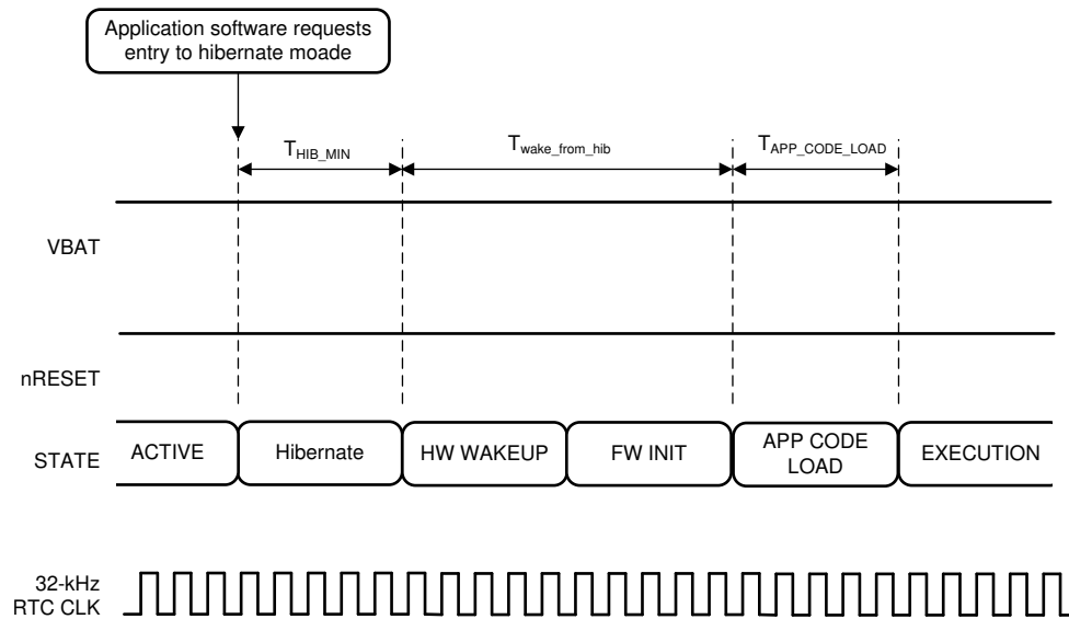
8-7. Wake Up From Hibernate Timing Diagram
