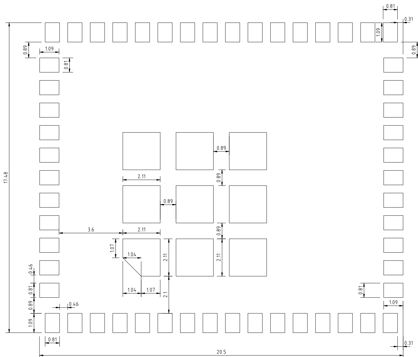
図 13-2. Land Pattern Drawing
