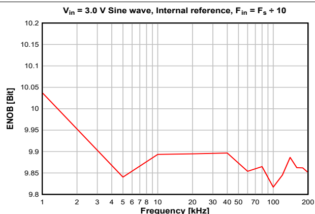
7-23. ENOB vs. Sampling Frequency
