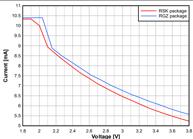
図 7-7. RX Current vs. Supply Voltage (VDD5) (BLE 1Mbps, 2.44GHz)
