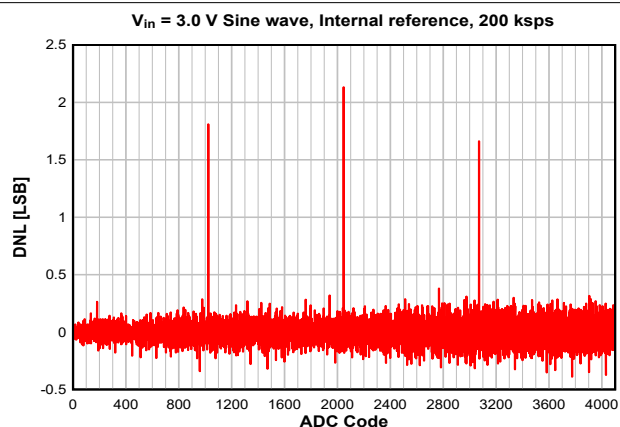
7-25. DNL vs. ADC Code
