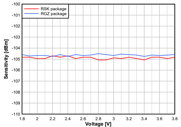
7-15. Sensitivity vs. Supply Voltage (VDD) (250kbps, 2.44GHz)
