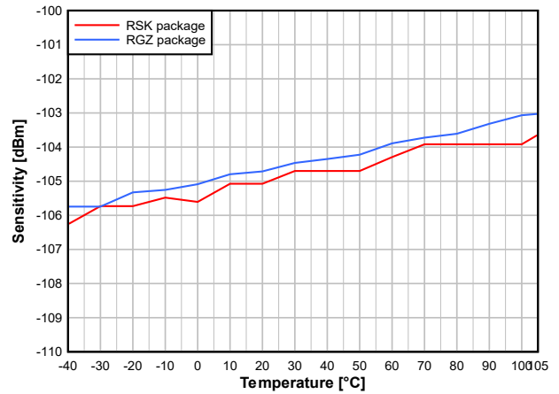
7-13. Sensitivity vs. Temperature (250kbps, 2.44GHz)
