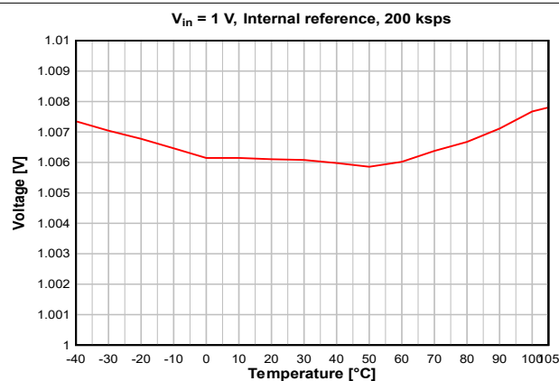
7-26. ADC Accuracy vs. Temperature
