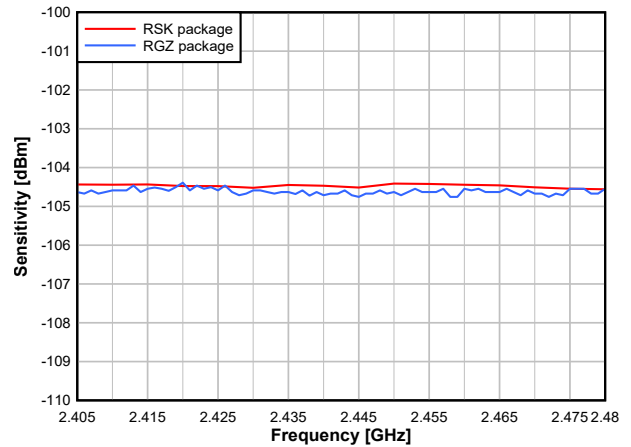
7-11. Sensitivity vs. Frequency (IEEE 802.15.4 OQPSK DSSS1:8, 250kbps, 2.44GHz)
