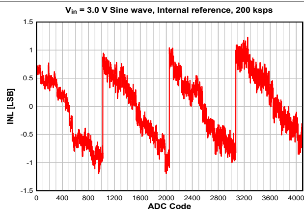
7-24. INL vs. ADC Code
