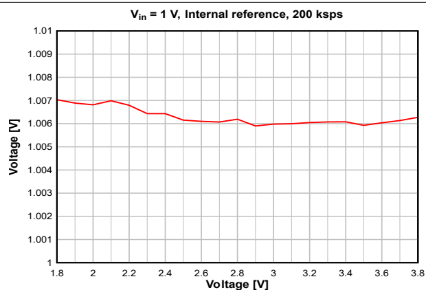
7-27. ADC Accuracy vs. Supply Voltage (VDD)
