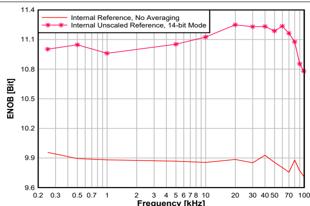
7-22. ENOB vs. Input Frequency
