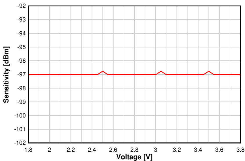
8-16. Sensitivity vs. Supply Voltage (VDD5) (BLE 1 Mbps, 2.44 GHz, DCDC Off)
