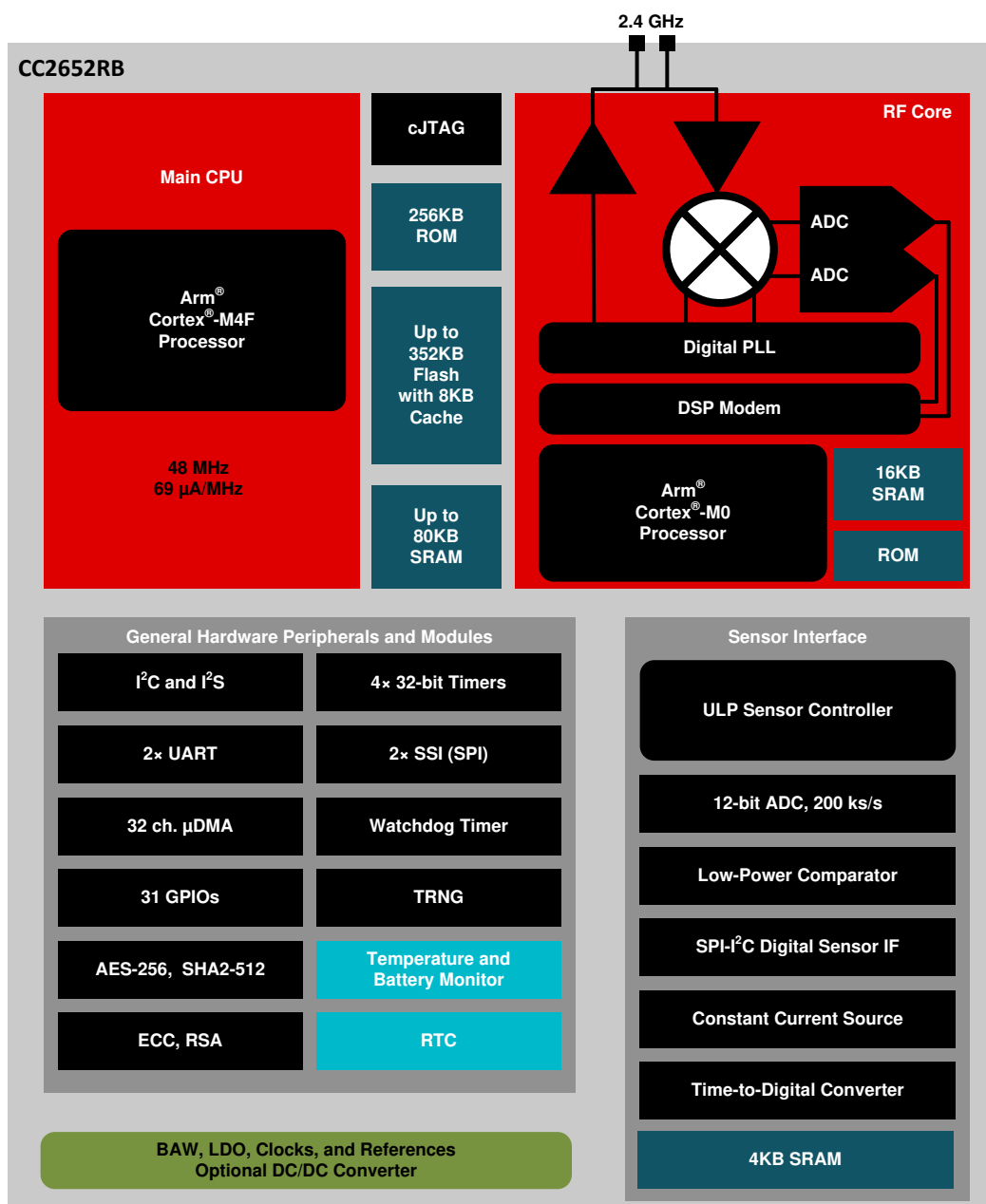
4-1. CC2652RB Block Diagram
