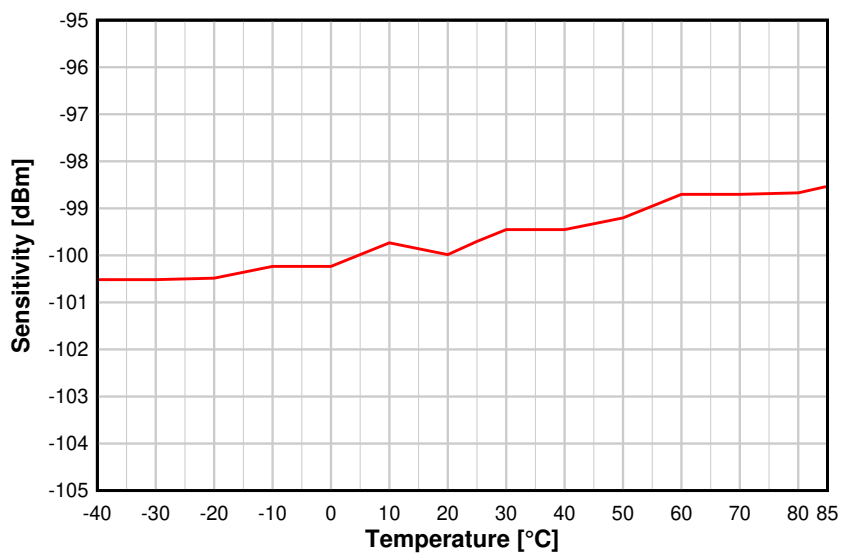
8-14. Sensitivity vs. Temperature IEEE 802.15.4 (OQPSK DSSS1:8, 250 kbps)
