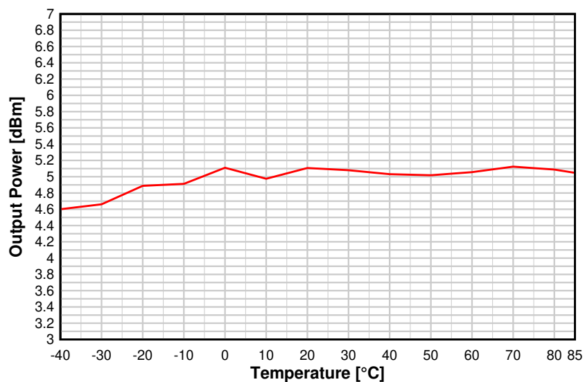
8-19. Output Power vs. Temperature (BLE 1 Mbps, 2.44 GHz, +5 dBm)
