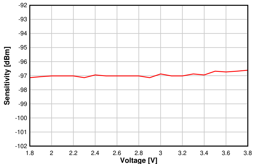
8-15. Sensitivity vs. Supply Voltage (VDD5) (BLE 1 Mbps, 2.44 GHz)
