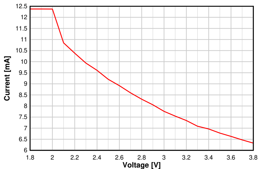
8-10. TX Current vs. Supply Voltage (VDDS) (BLE 1 Mbps, 2.44 GHz)
