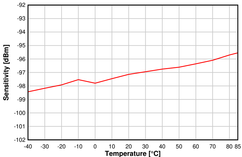
8-13. Sensitivity vs. Temperature (BLE 1 Mbps, 2.44 GHz)
