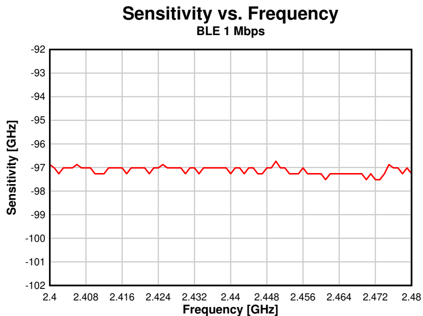
8-11. Sensitivity vs. Frequency (BLE 1 Mbps, 2.44 GHz)
