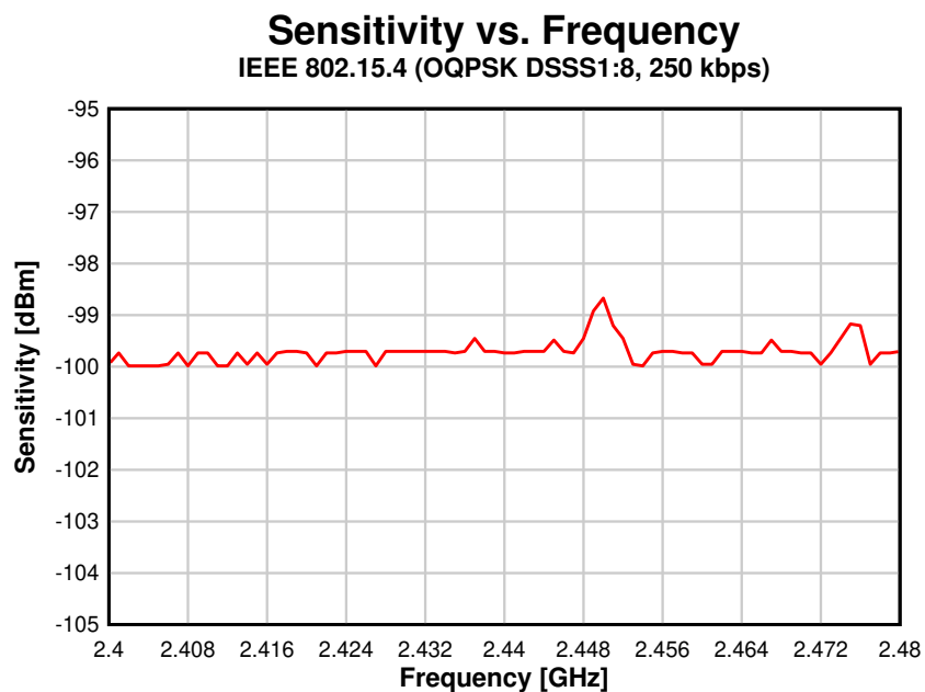
8-12. Sensitivity vs. Frequency IEEE 802.15.4 (OQPSK DSSS1:8, 250 kbps)
