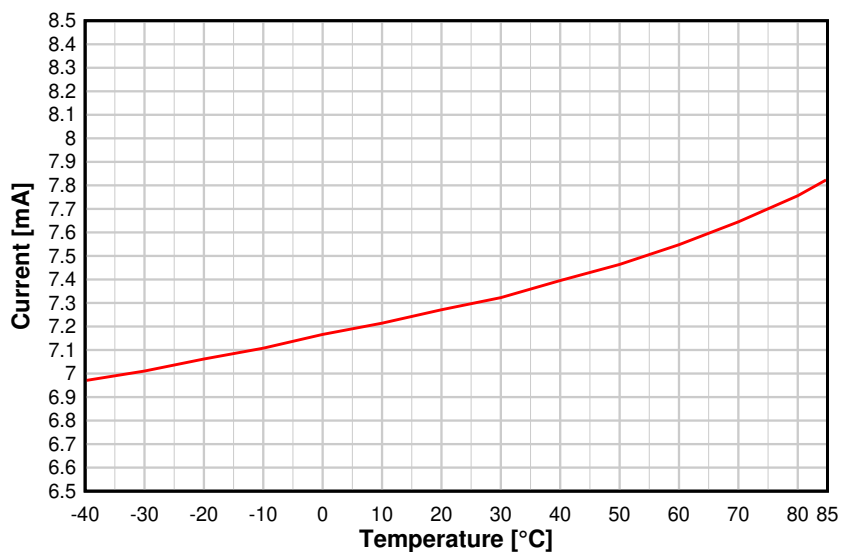
8-7. RX Current vs. Temperature (BLE 1 Mbps, 2.44 GHz)
