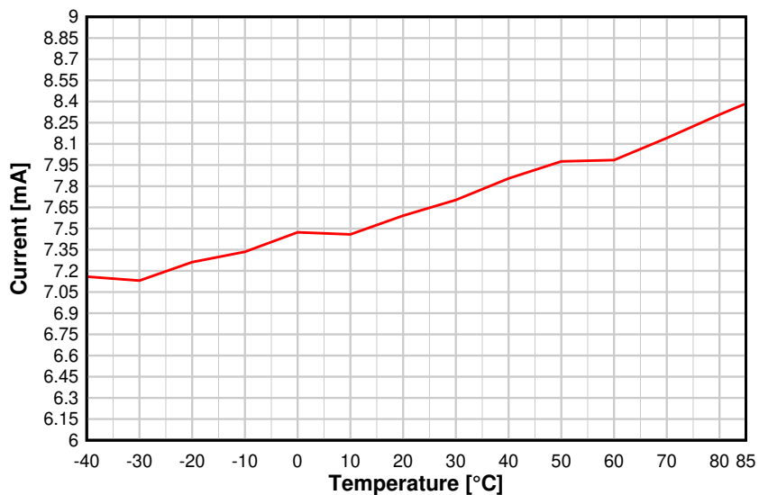
FIG 8-9. TX Current vs. Temperature (BLE 1 Mbps, 2.44 GHz)
