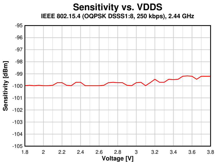
8-17. Sensitivity vs. Supply Voltage (VDD) IEEE 802.15.4 (OQPSK DSSS1:8, 250 kbps)
