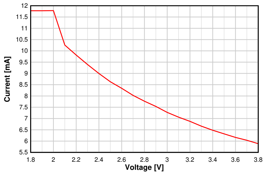
8-8. RX Current vs. Supply Voltage (VDD5) (BLE 1 Mbps, 2.44 GHz)
